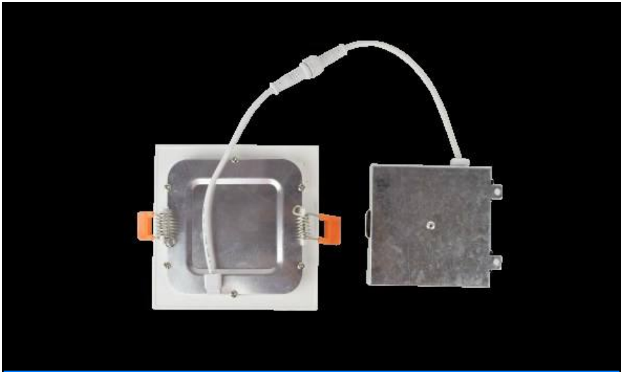
GL-SFS-S3 SHADE Aluminum Alloy · Slim Square 3" DIM Cut 75 × 75 mm LAMP SMD2835 6W LED 6W · 420LM · Dimmable
