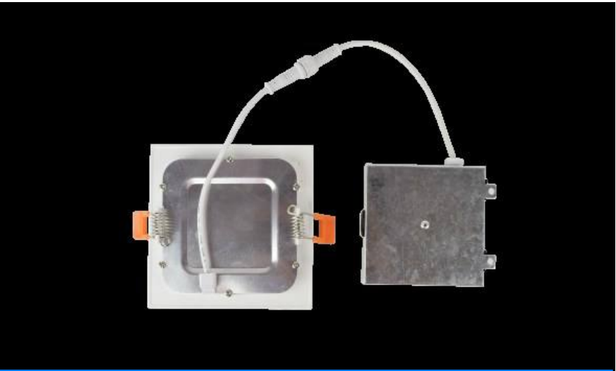
GL-SFS-S6 SHADE Aluminum Alloy · Slim Square 6" DIM Cut 156 × 156 mm LAMP SMD2835 15W LED 15W · 1125LM · Dimmable
