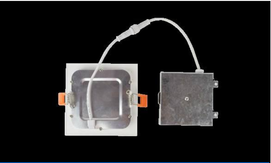
GL-SFS-S5 SHADE Aluminum Alloy · Slim Square 5" DIM Cut 135 × 135 mm LAMP SMD2835 12W LED 12W · 900LM · Dimmable
