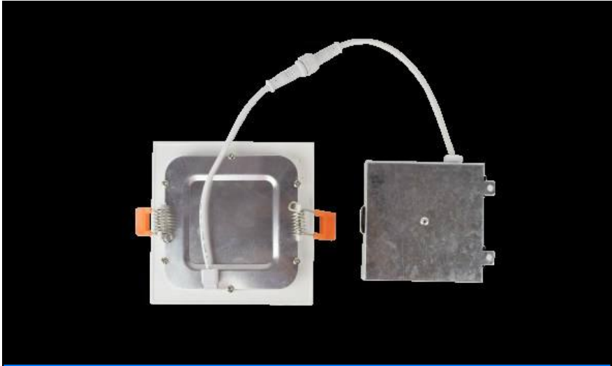
GL-SFS-S8 SHADE Aluminum Alloy · Slim Square 8" DIM Cut 185 × 185 mm LAMP SMD2835 18W LED 18W · 1350LM · Dimmable
