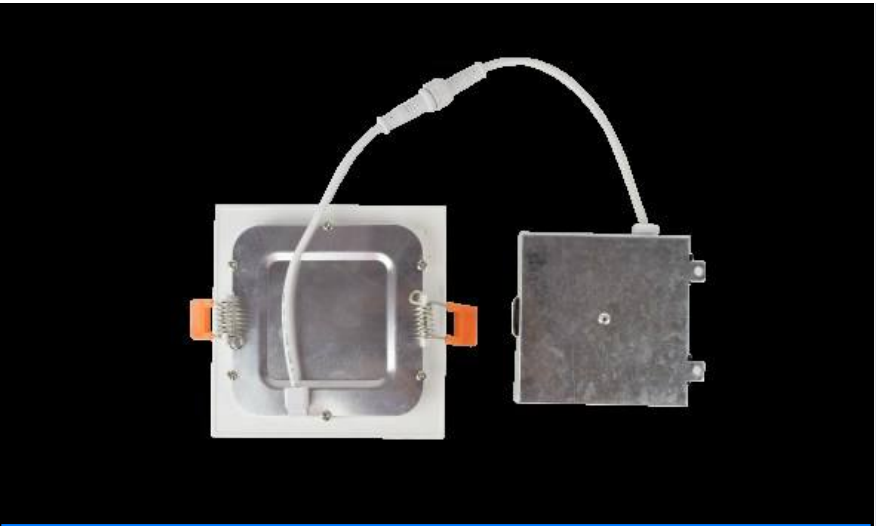
GL-SFS-S4 SHADE Aluminum Alloy · Slim Square 4" DIM Cut 110 × 110 mm LAMP SMD2835 9W LED 9W · 630LM · Dimmable
